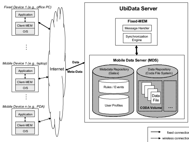
Figure 1: Conceptual Overview of the UbiData Architecture.
